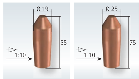
Electrode PPS 35/60
